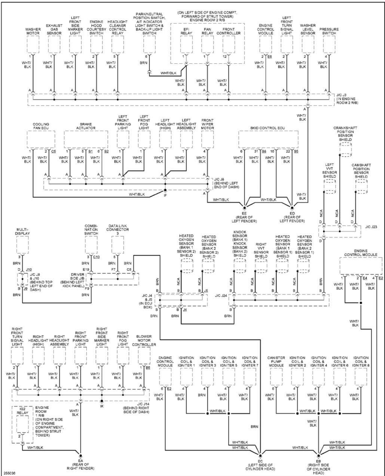
Fig. 28: Ground Distribution Circuit (2 of 3)
