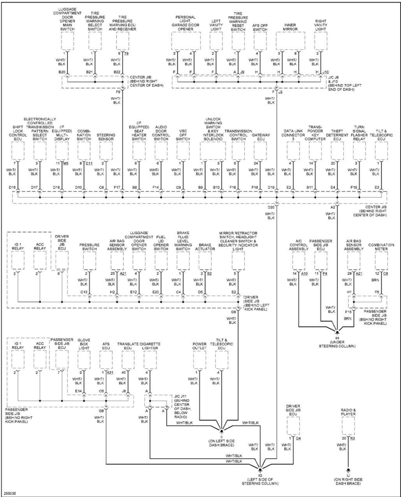
Fig. 27: Ground Distribution Circuit (1 of 3)
