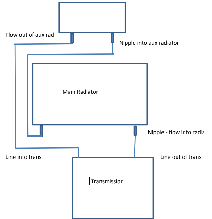
ADDING AUX TRANS COOLING RADIATOR
