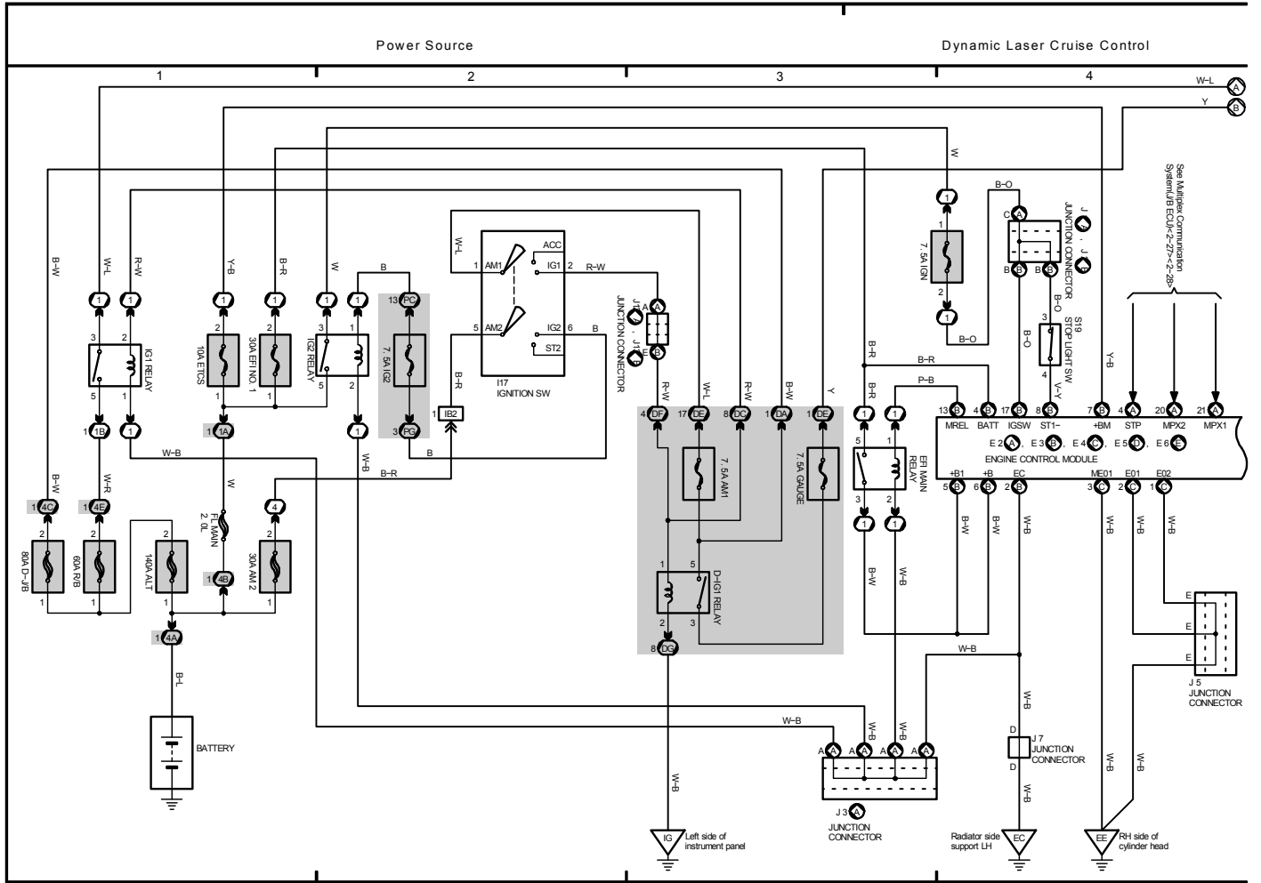
OVERALL ELECTRICAL WIRING DIAGRAM
