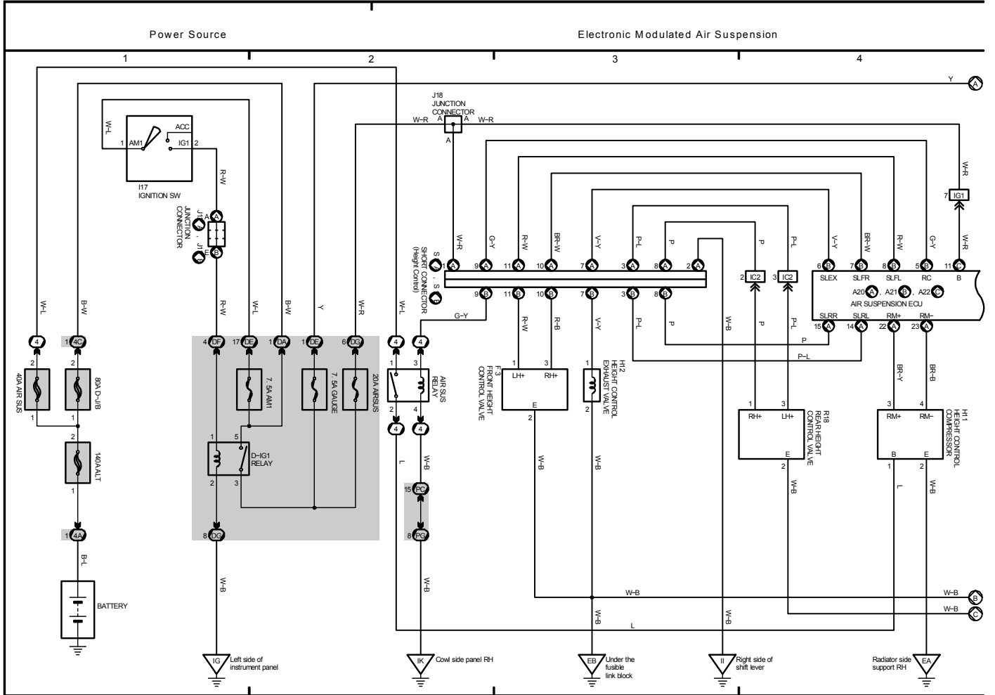
M OVERALL ELECTRICAL WIRING DIAGRAM
