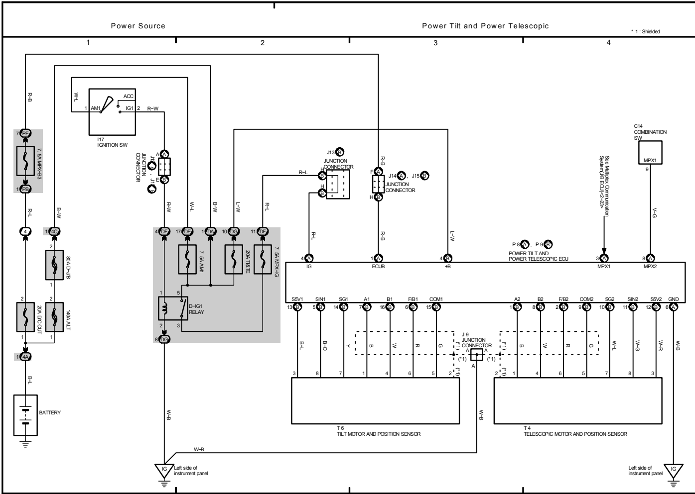
M OVERALL ELECTRICAL WIRING DIAGRAM
