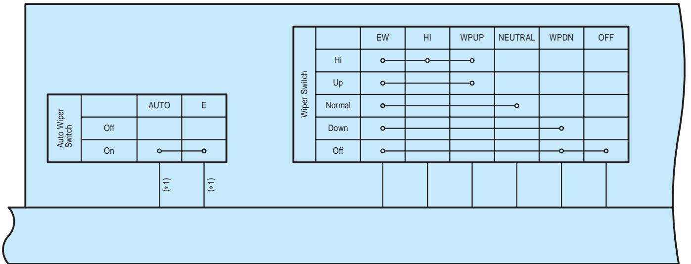
K24(A), K25(B) Windshield Wiper Switch Assembly
