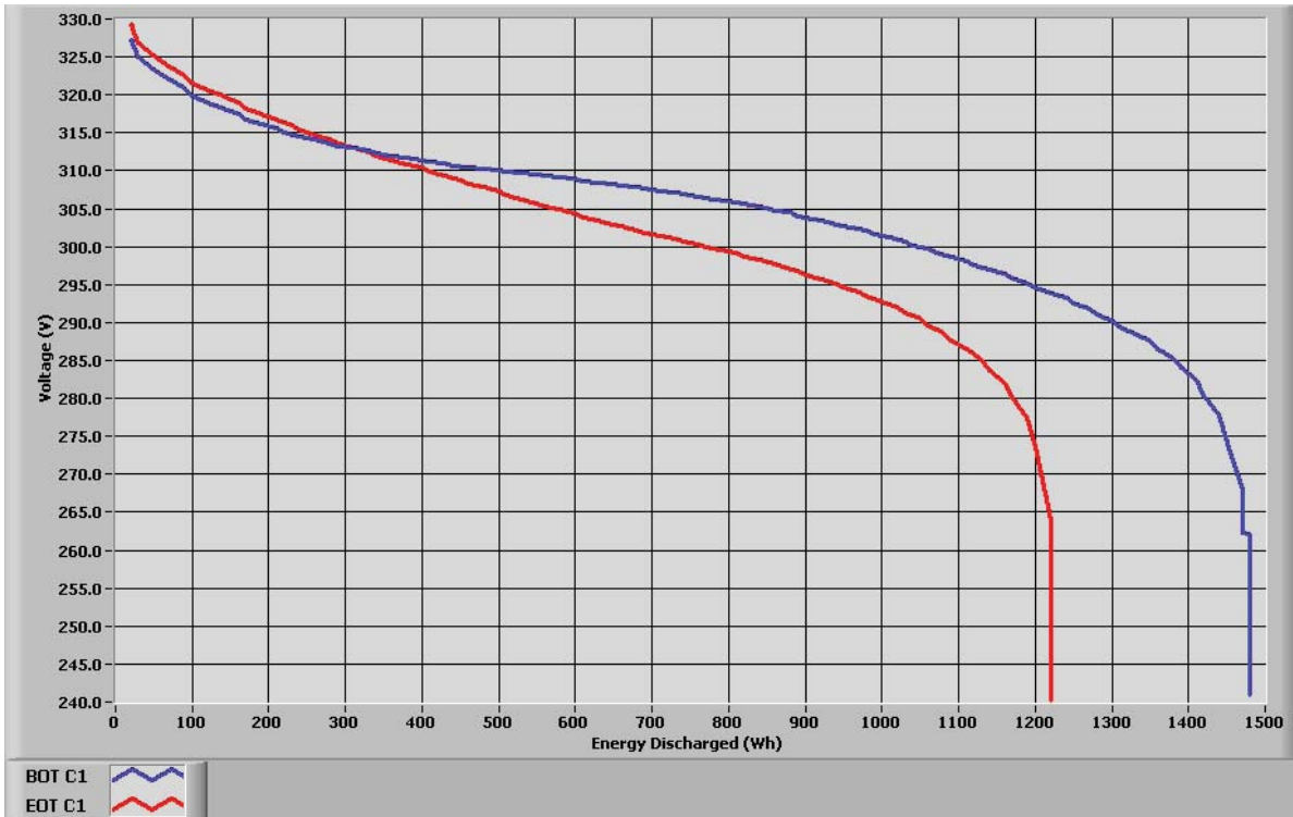
Figure 1. Voltage versus energy discharged.
