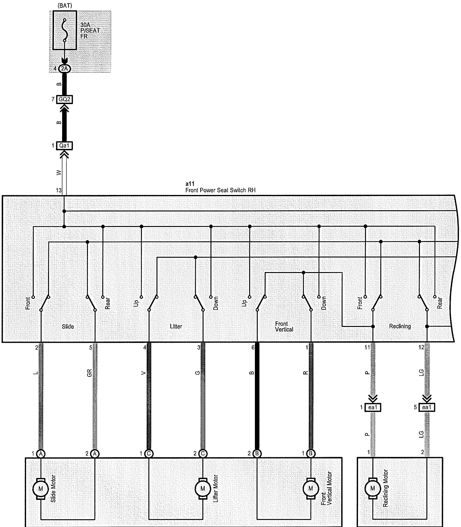
a8(A), a9(B), a10(C) Separate Type Front Seat Cushion Spring Assembly RH
