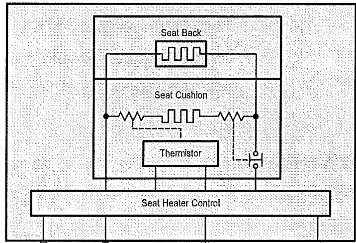
a13 Front Seat Heater Assembly RH
