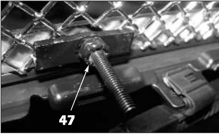
47. Paint the #8 - 32 ESNA half nuts and mounting studs across the bottom of the upper mesh grille assembly.
