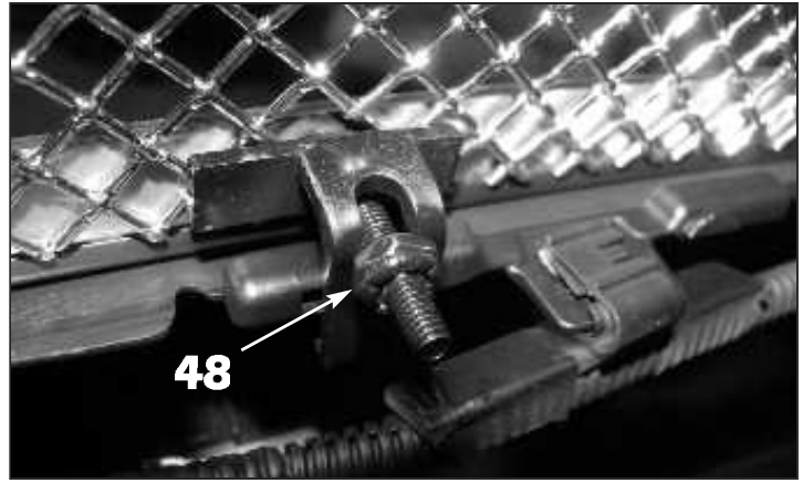
48. Align the universal U-shaped mesh retainers onto each of the bottom mounting studs and tighten until the lower portion of the grille is flush against the bumper cover. Once tight, paint the #8-32 ESNA half nuts and the exposed threads of the mounting studs black.
