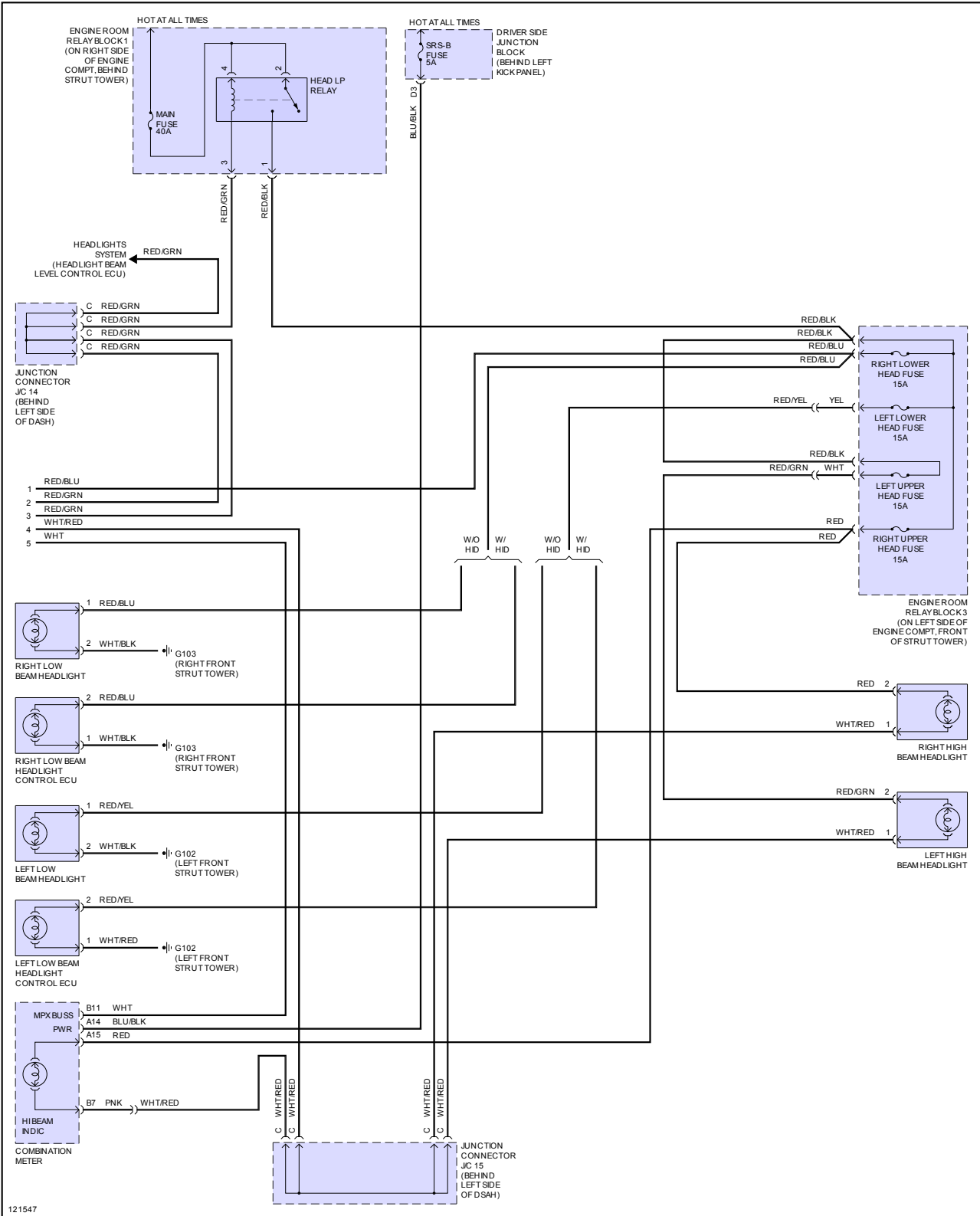
Fig 4: Headlamps Circuit, W/O DRL (2 of 2)
