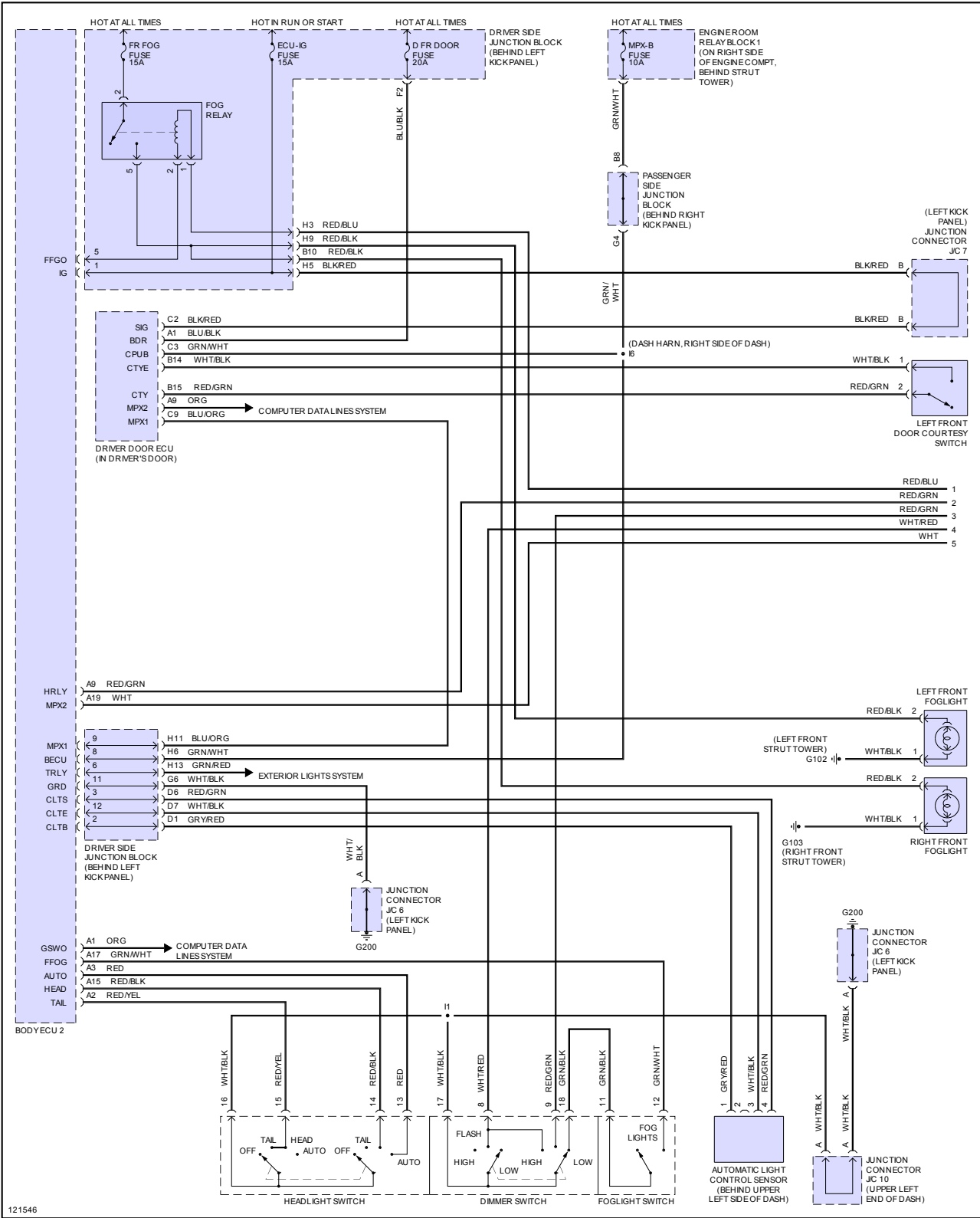
Fig 3: Headlamps Circuit, W/O DRL (1 of 2)
