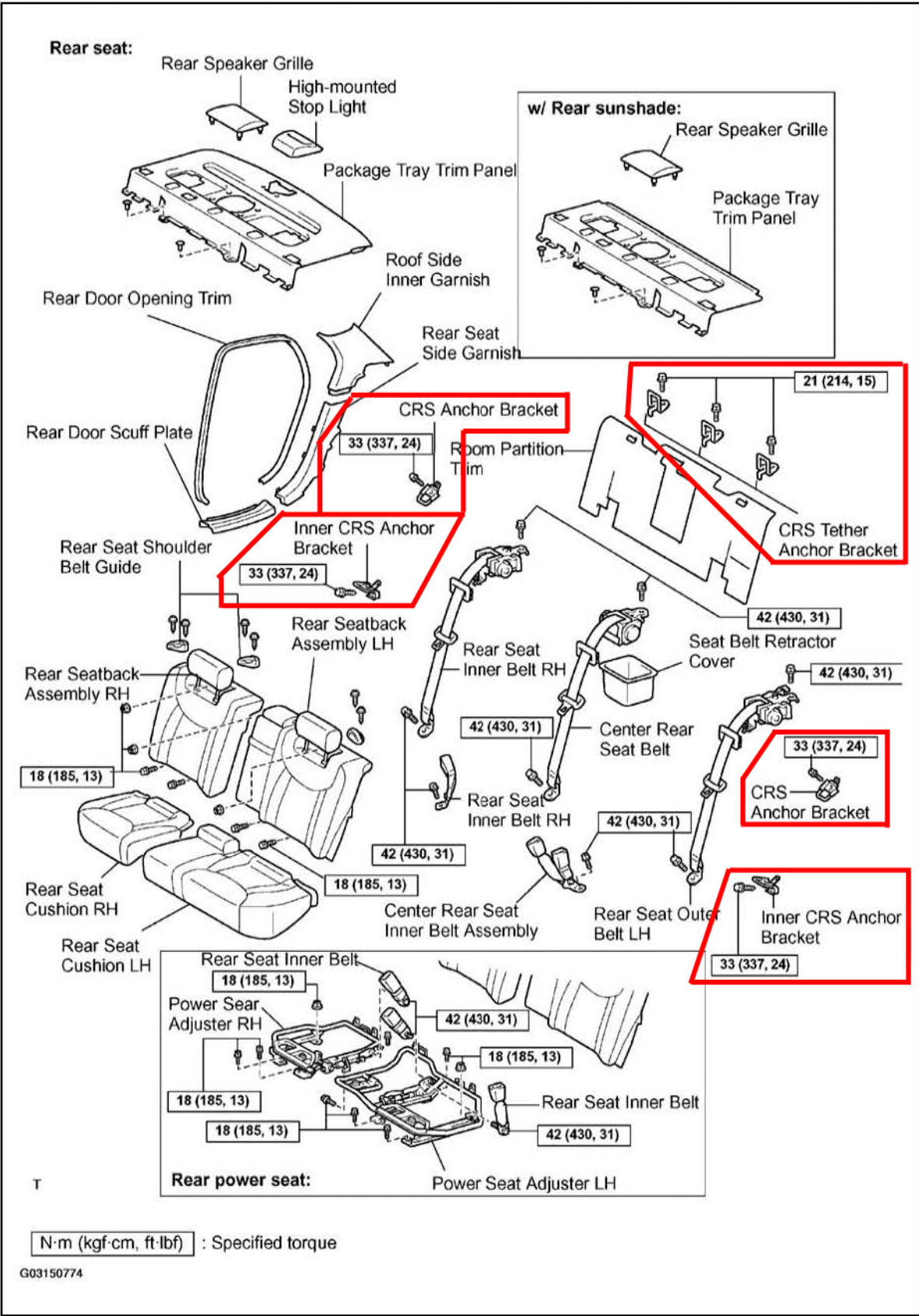
Fig 2: Identifying Components For Seat Belt Removal (Back Seat)
